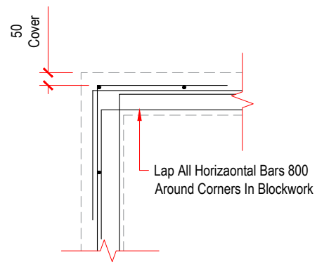
6 Detail SCALE 1: 30
