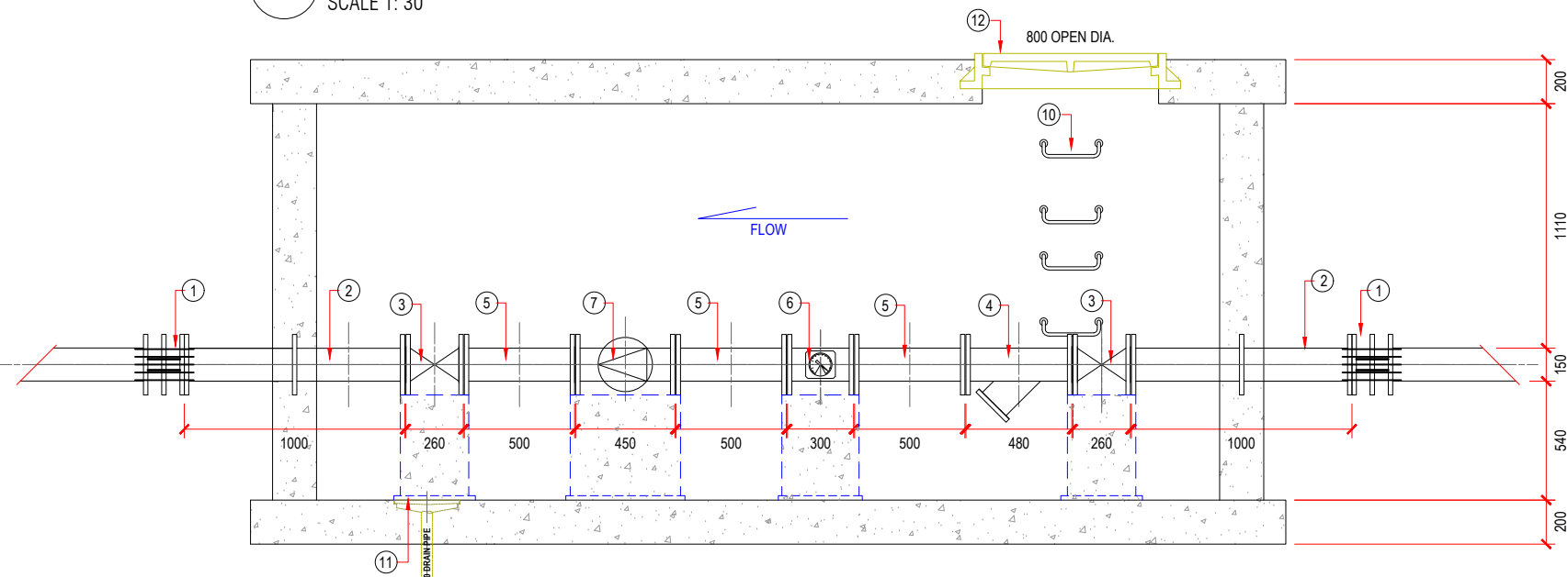
1 Section A - A SCALE 1: 30
