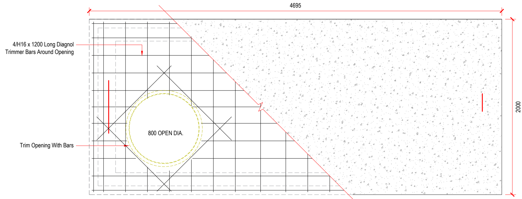
3 Precast Lid Panel Plan SCALE 1: 30
