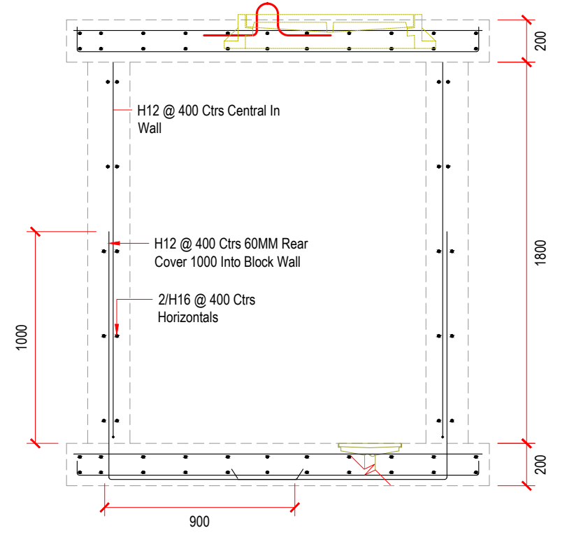
5 Cross Section SCALE 1: 30
