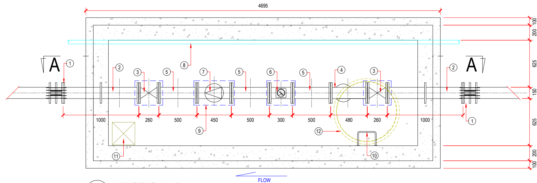
1 150MM Ø PRV Chamber Plan SCALE 1: 30
