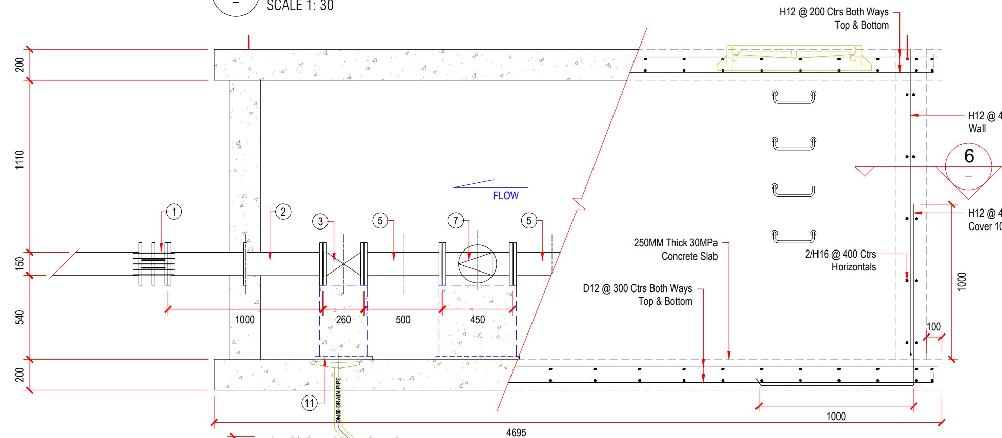
4 Cross Section SCALE 1: 30
