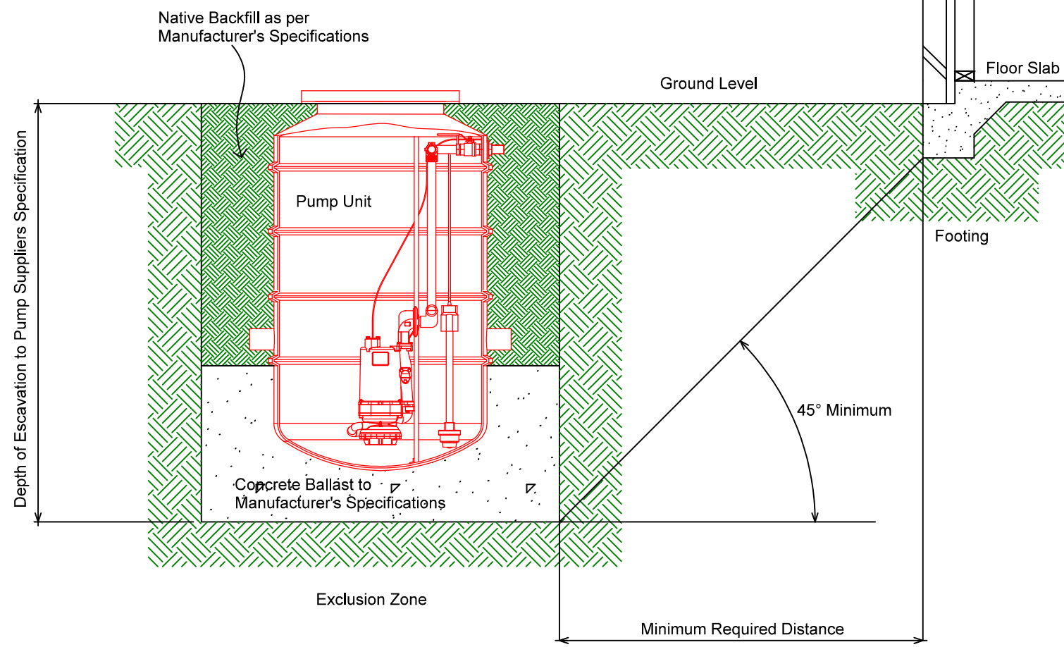
Typical Pump Unit Surround Plinth
