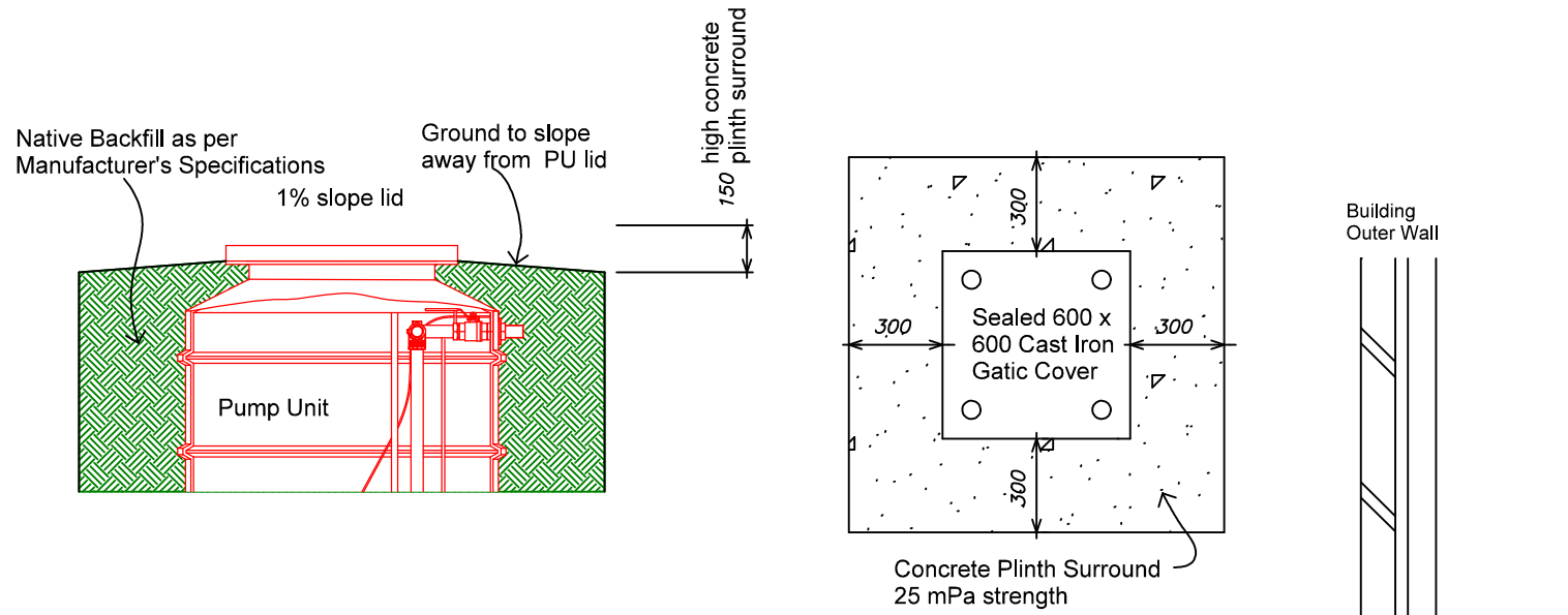
Typical Pump Unit Surround Plinth
